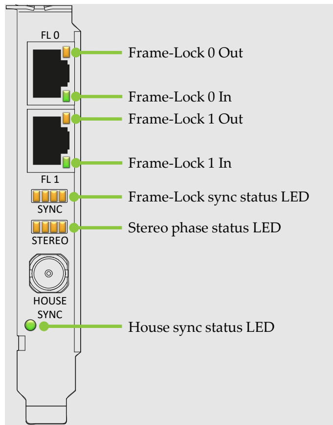
Figure 6. Board Level Status Indicators
