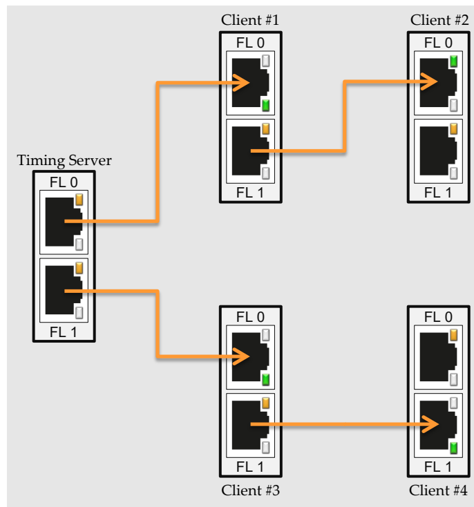
Figure 4. FrameLock Connections on Timing Server
